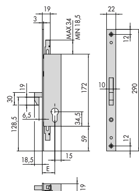
46260, 46262 E = 25 - 30 - 35
