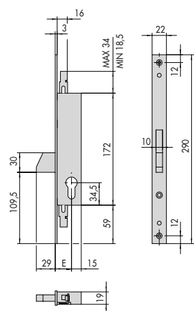
46220, 46222 E = 25 - 30 - 35
