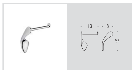
B1808 Porta rotolo Paper holder
