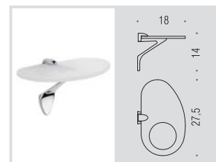
B1803 Porta sapone da vasca Soap dish for bath
