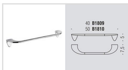
B1809 - B1810 Porta salvietta Towel holder
